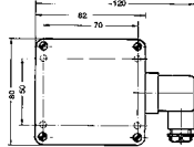
Dimensioned sketch GPHU / GRMU:
